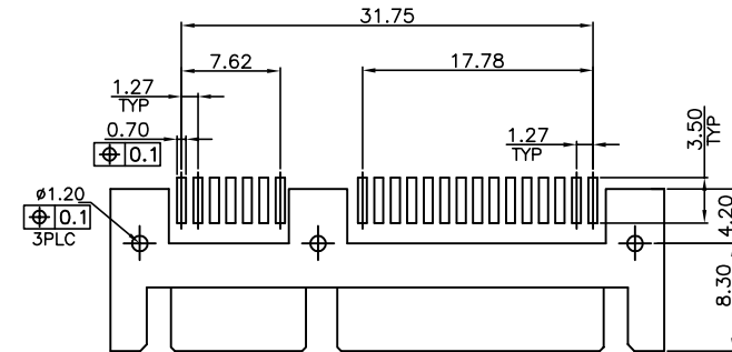
PCB LAYOUT RECOMMENDED PCB TOLERANCE:±0.05
