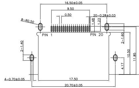
RECOMMENDED PCB LAYOUT(TOP VIEW) (TOLERANCE=±0.03mm)
