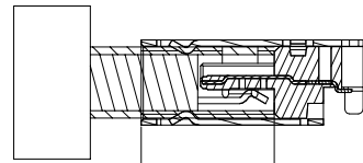
PLUG Fully Insert
