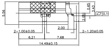
PLUG Fully Insert
