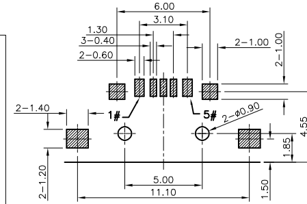
RECOMMENDED P.C.B. LAYOUT (TOP VIEW) GENERAL TOLERANCE: ±0.05
