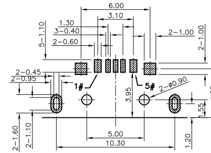
RECOMMENDED P.C.B. LAYOUT (TOP VIEW) GENERAL TOLERANCE: ±0.05
