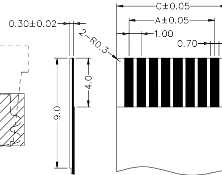
PROPER CABLE (SCALE 2:1)
