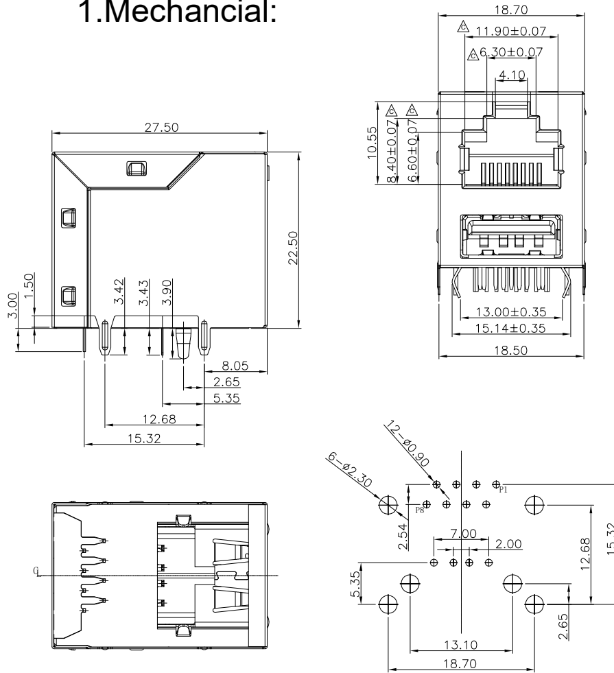
RECOMMENDED P.C.B LAYOUT TOP VIEW (COMPONENT SIDE)
