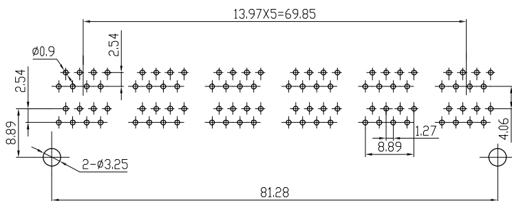
PCBLAYOUT
