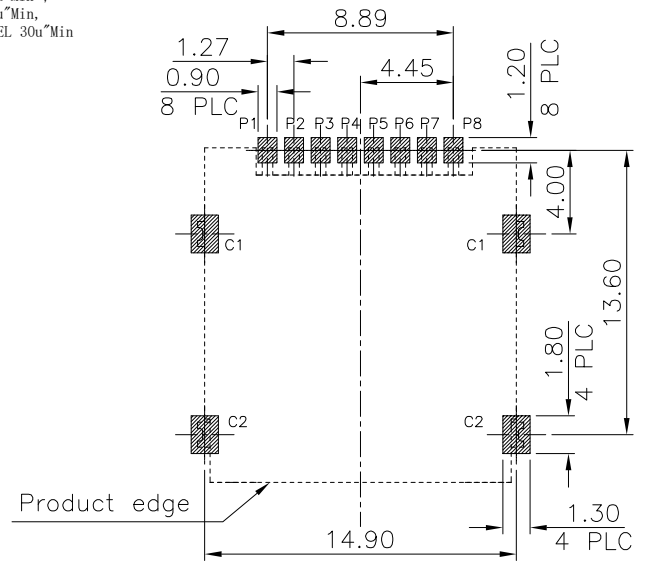
RECOMMENDED PCB LAYOUT(TOP VIEW) GENERAL TOLERANCES: ±0.05
