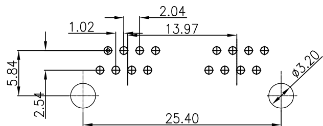
PCBLAYOUT TOL:±0.05
