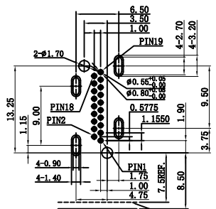
RECOMMENDED PCB LAYOUT (TOP VIEW) TOLERANCE: ±0.05mm
