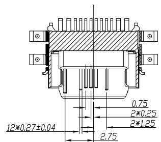
SEC B-B
