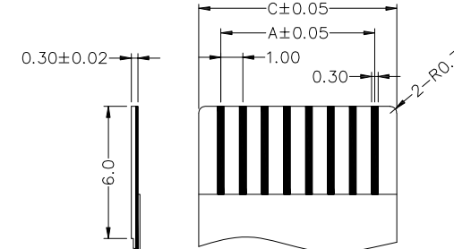
PROPER CABLE (SCALE 2:1)
