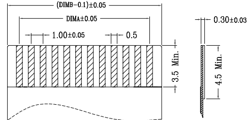
通用扁平线 (Applicable Flat Cable)
