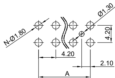
P.C.B LAYOUT(TOP VIEW) TOLERANCE:±0.10
