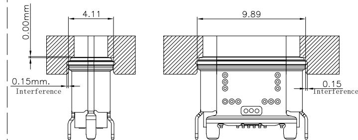
RECOMMENDED CAVITY "2" SIZE
