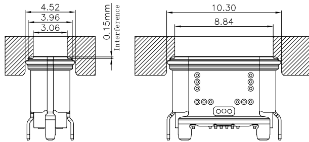
RECOMMENDED CAVITY "1" SIZE
