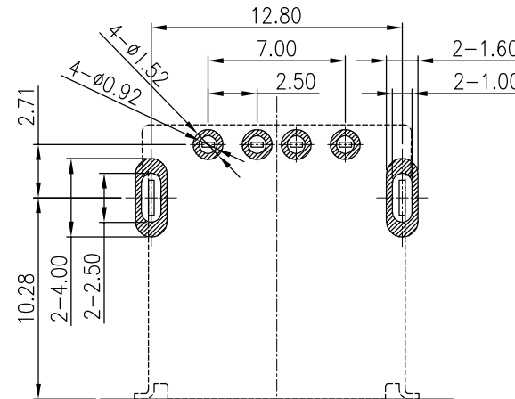
RECOMMENDED P.C.B HOLE LAYOUT TOP VIEW(TOLERANCE:±0.08)
