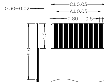
PROPER CABLE (SCALE 2:1)
