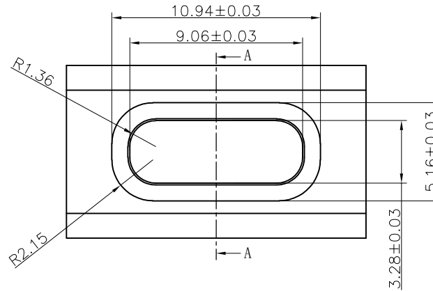
机壳开孔尺寸图 SIZE DRAWING OF OPENING HOLE OF HOUSING
