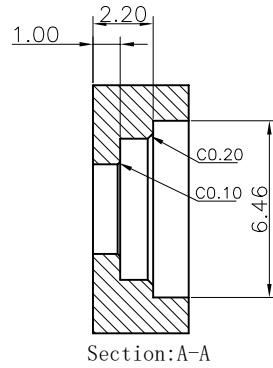
机壳开孔尺寸图 SIZE DRAWING OF OPENING HOLE OF HOUSING
