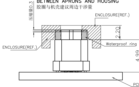
RECOMMENDED SCHEMATIC DRAWING OF CONNECTOR MATCH CHASSIS
