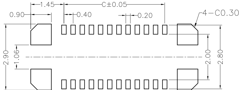
RECOMMENDED PCB LAYOUT CONNECTOR SIDE
